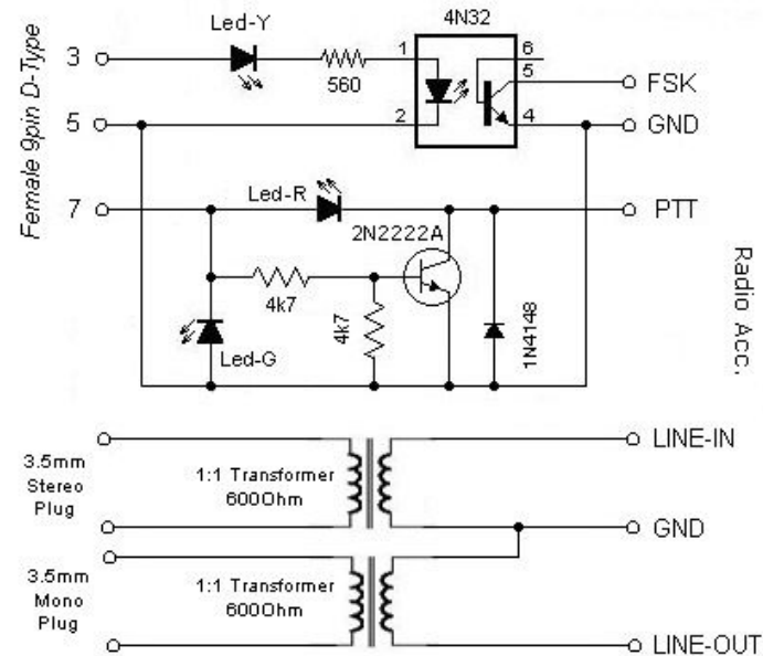
Digital Interface with FSK
