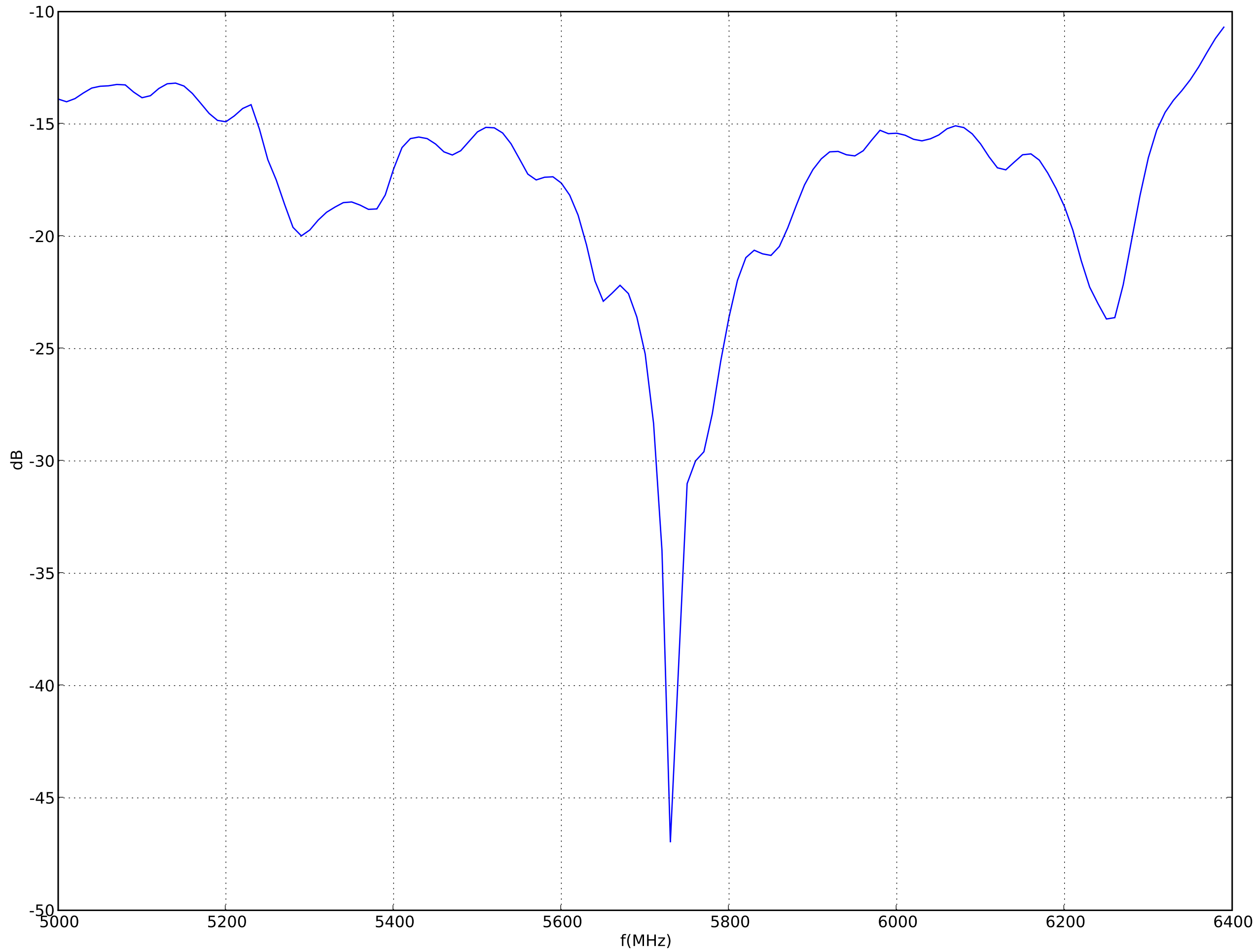
SQG 5.7 GHz return loss - Narda coupler
